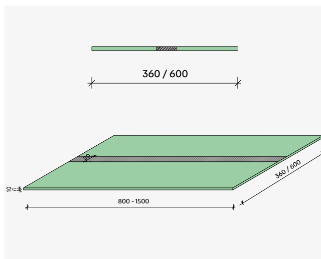
Dimensions SINTON® ZB - Allocation with line bearing
