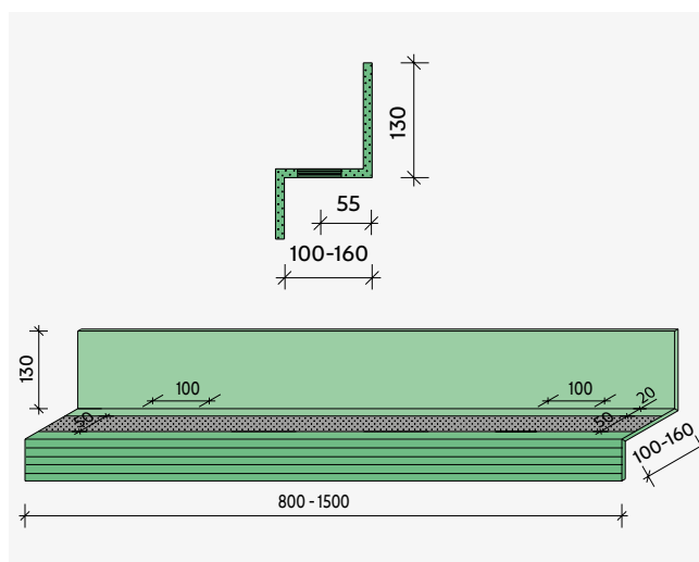
Dimensions SINTON® Z - Allocation with line bearing
