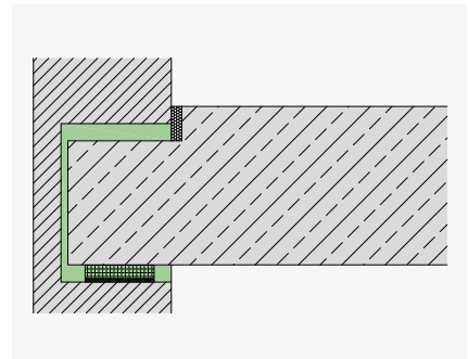
Landing height h > 180 mm
