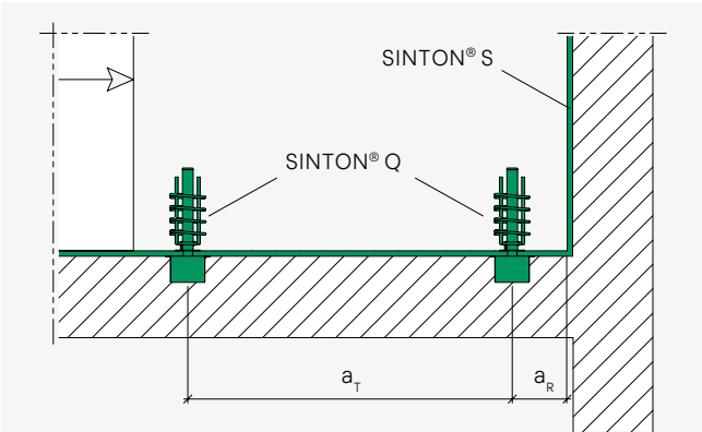
Element arrangement SINTON® Q in the pedestal: Center distance a T
