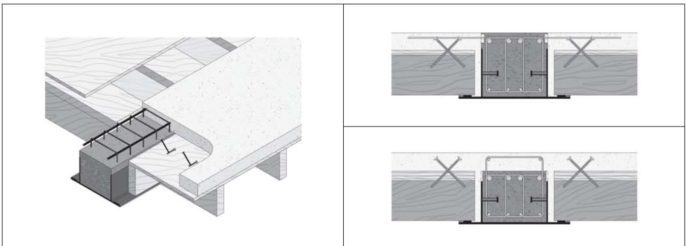
Timber-concrete composite floors (wet concrete part). Ribs made of timber.
