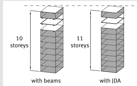
Lower construction height with JORDAHL® JDA punching shear reinforcement
